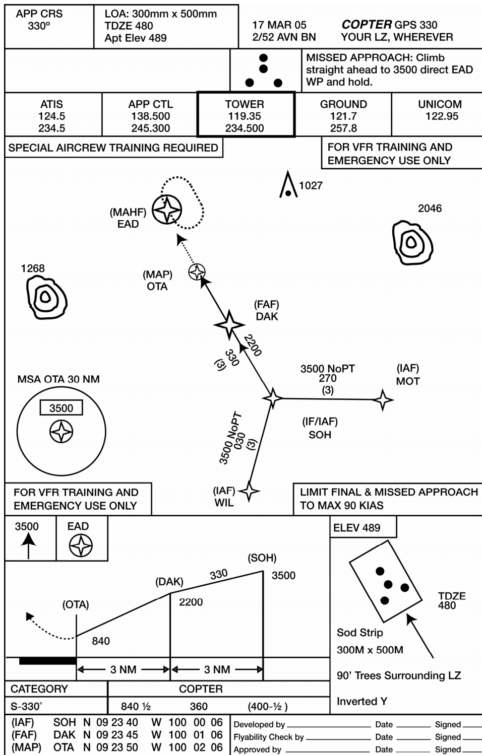
Figure 4-8. Sample of an emergency GPS recovery procedure diagram
